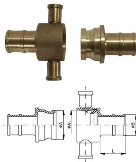
BS336 Coupling in Brass & Aluminuim
