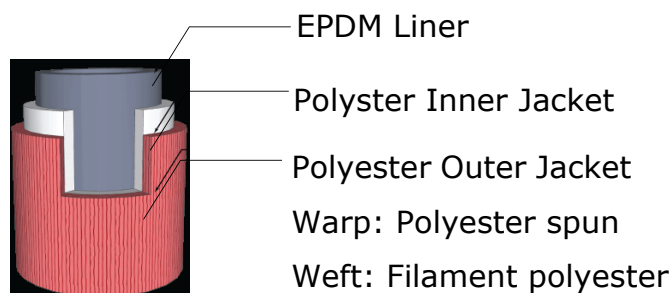
Double Jacket Hose
